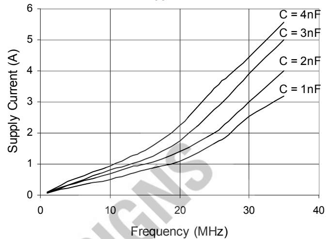
Fig. 11 Supply Current vs. Load Capacitance V_{CC} = 8V
