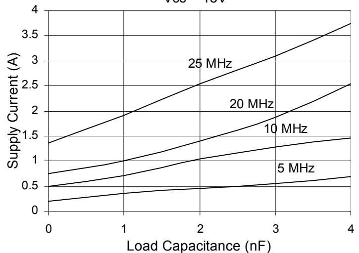
Fig. 13 Supply Current vs. Load Capacitance V_{CC} = 15V
