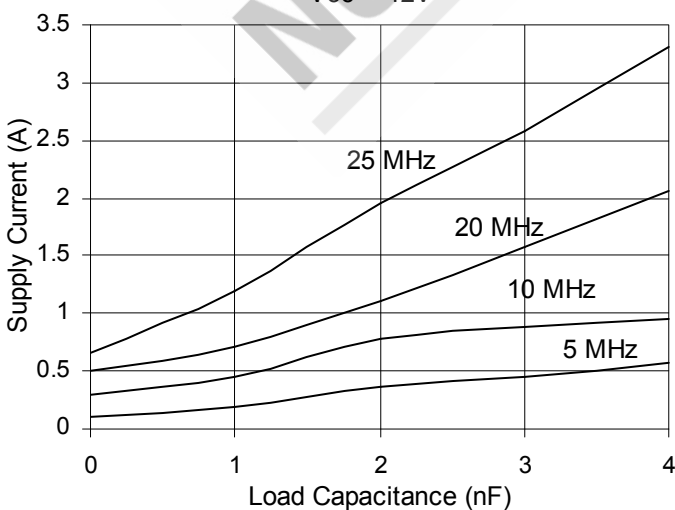
Fig. 12 Supply Current vs. Load Capacitance V_{CC} = 12V
