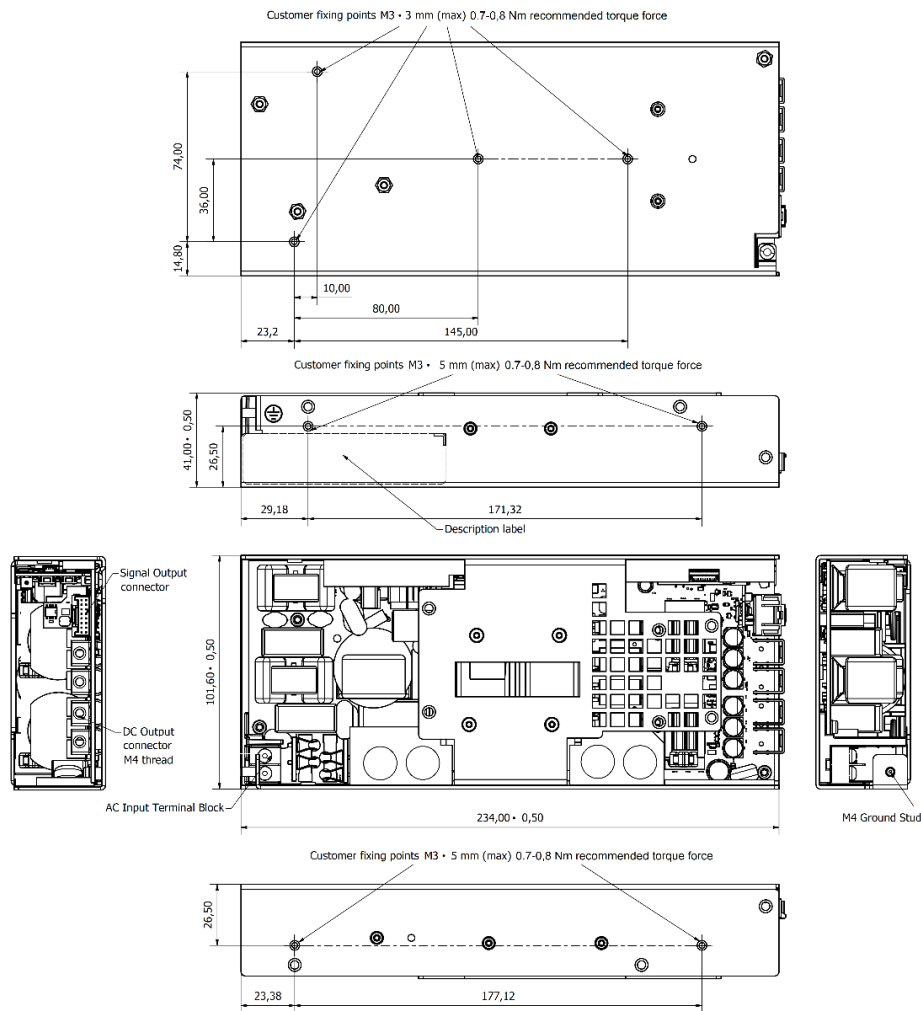
Figure 1. Mechanical Drawing - ABC1200-1T24-UCF Model
