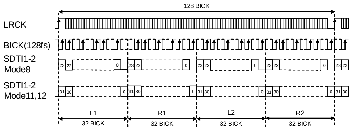
Figure 24. Mode 8/11/12 Timing
