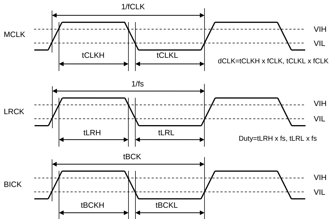
Figure 10. Clock Timing
