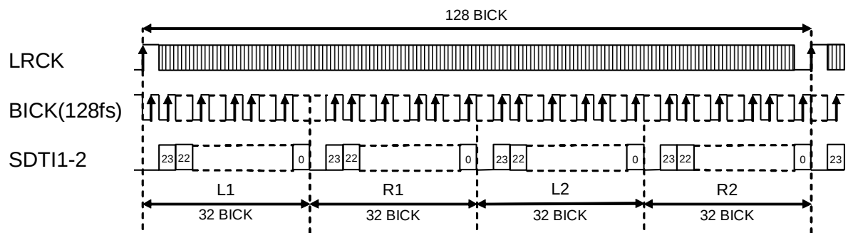
Figure 26. Mode 10 Timing
