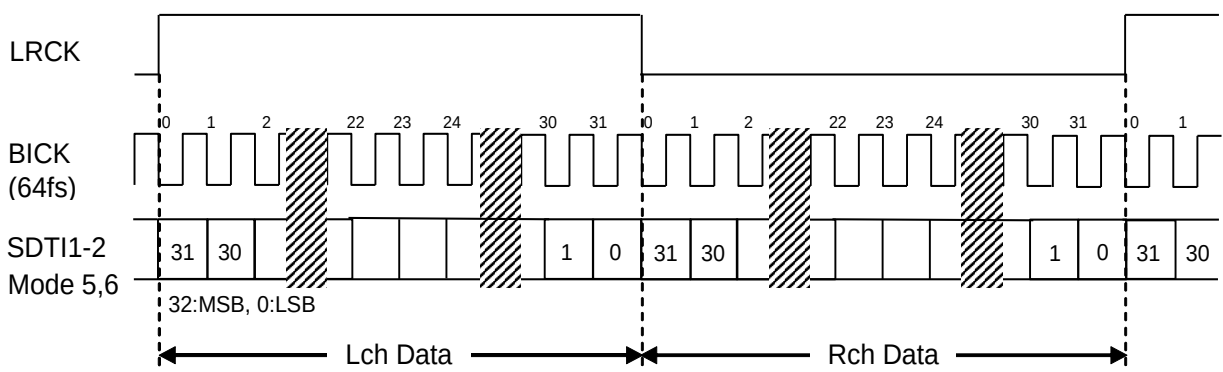
Figure 22. Mode 5/6 Timing
