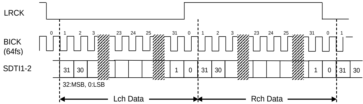
Figure 22. Mode 5/6 Timing
