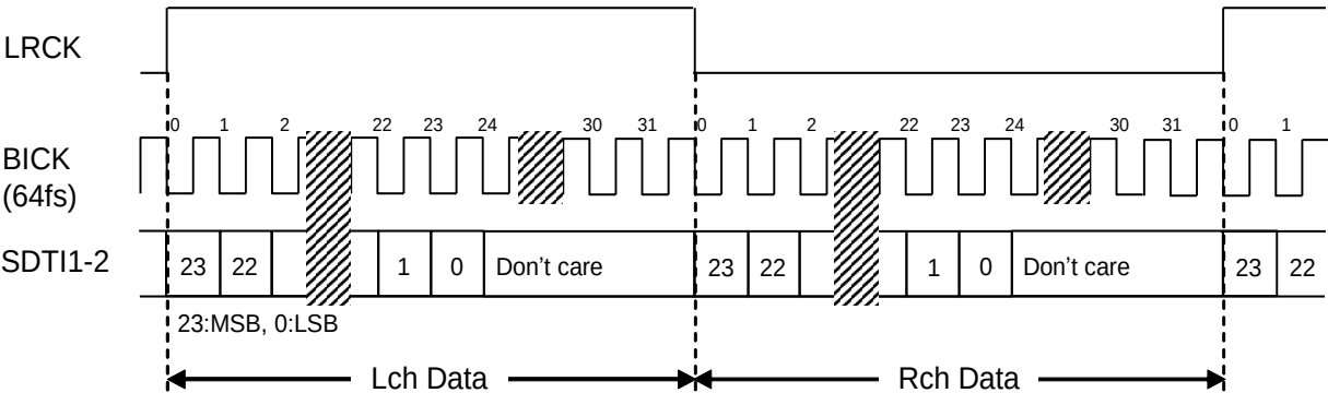
Figure 20. Mode 2 Timing
