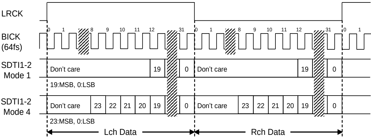
Figure 19. Mode 1/4 Timing
