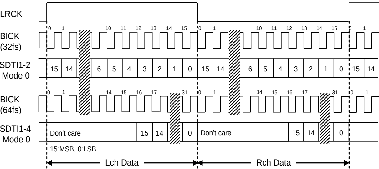
Figure 18. Mode 0 Timing
