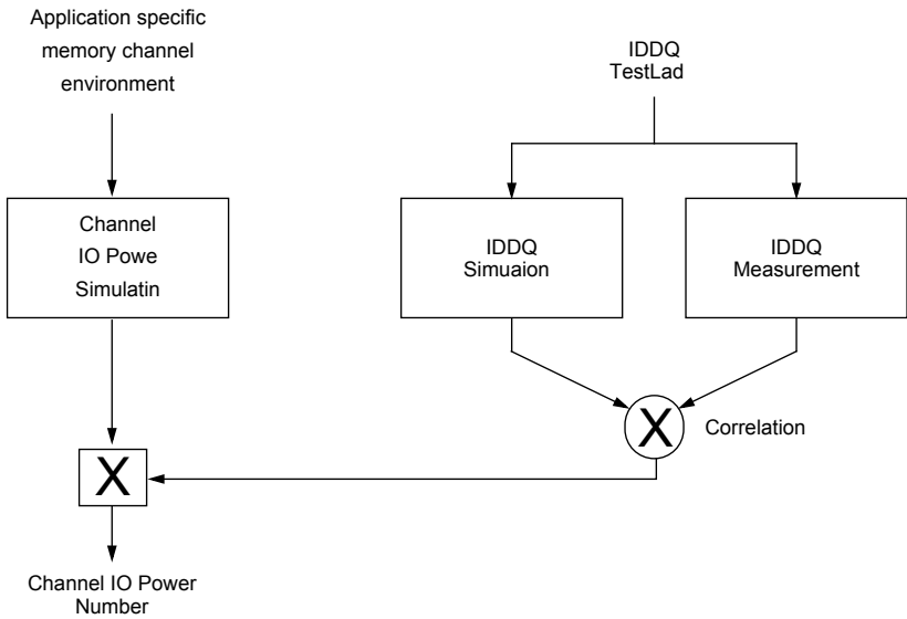
Figure 20. Correlation from simulated Channel IO Power to actual Channel IO Power supported by IDDQ Measurement.
