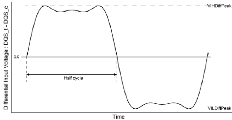
Figure 10. Definition of differential DQS Signal AC-swing Level
