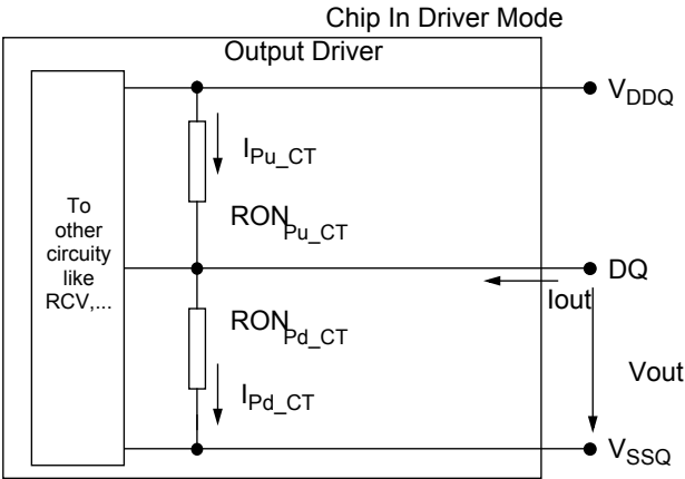
Figure 14. Output Driver
