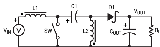
20a. SEPIC Topology
