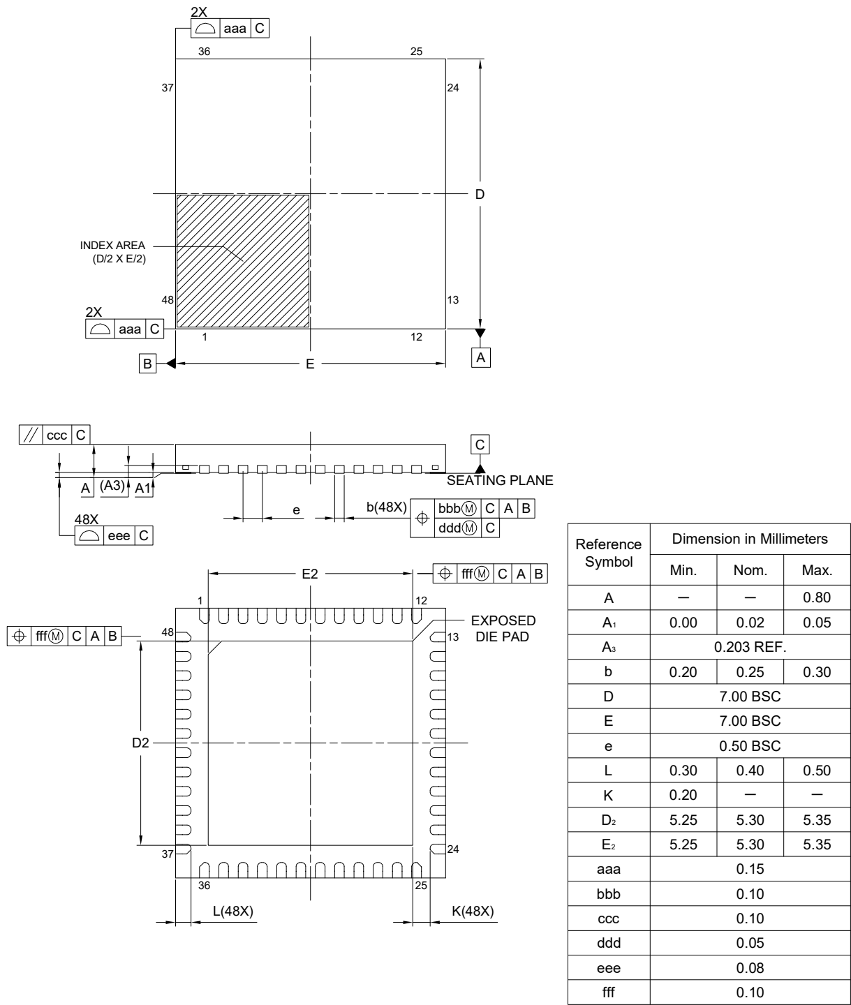
Figure A2.2 HWQFN 48-pin
