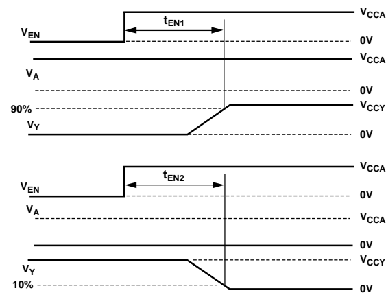
Figure 32. Enable Time
