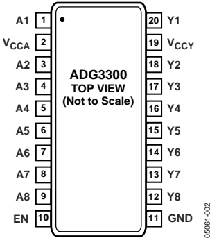
Figure 2. Pin Configuration
