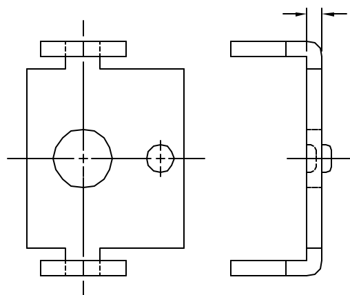
LOCK TAB
