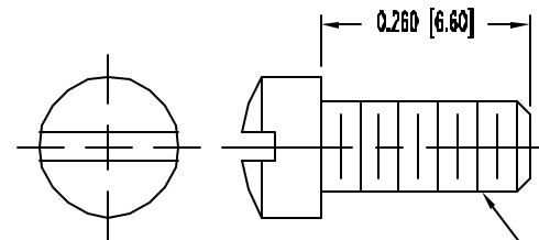
SCREW
