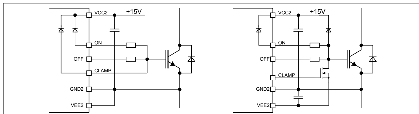
Figure 22 Short circuit clamping circuitry
