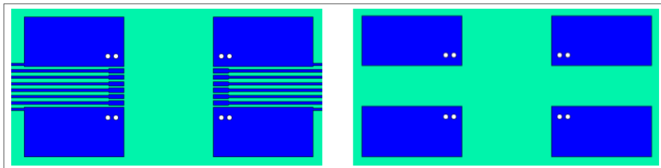
Figure 23 Reference layout for thermal data (Two layer PCB; copper thickness 35 μm; left: top layer; right: bottom layer)
