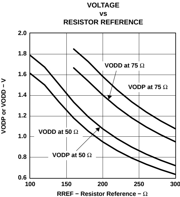
Figure 10. Differential Transmitter Voltage
