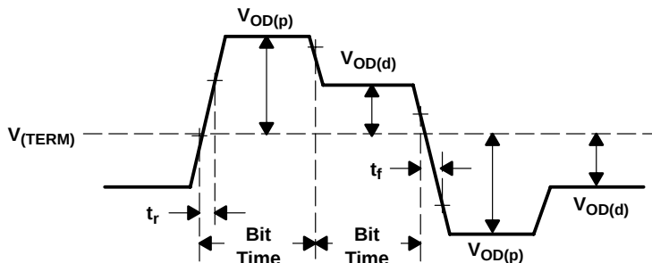
Figure 8. Differential and Common-Mode Output Voltage Definitions
