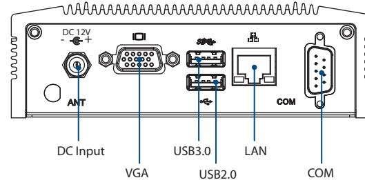
Rear Panel External I/O Mechanical Layout/Drawing
