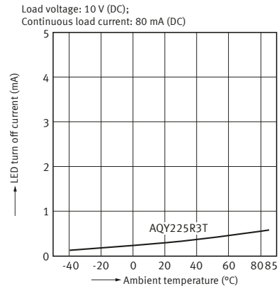
6-2. LED turn off current vs. ambient temperature characteristics
