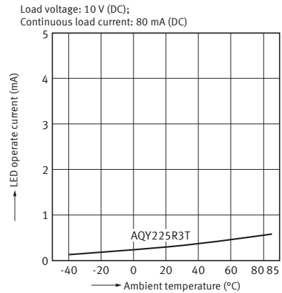
5-2. LED operate current vs. ambient temperature characteristics
