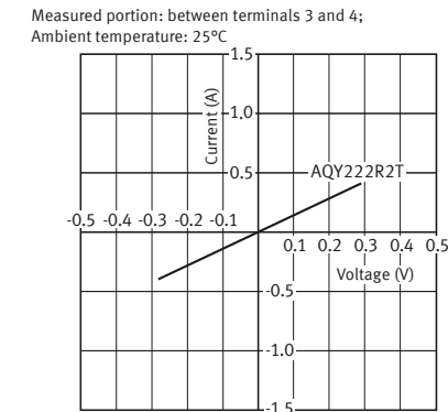
8-1. Current vs. voltage characteristics of output at MOS portion
