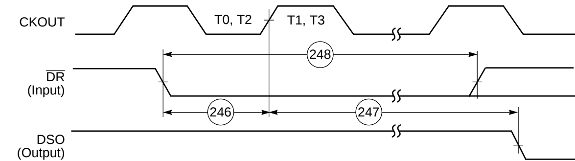
Figure 2-34 Synchronous Recovery from Wait State
