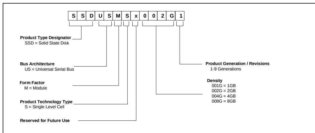
Figure 10. Decoder
