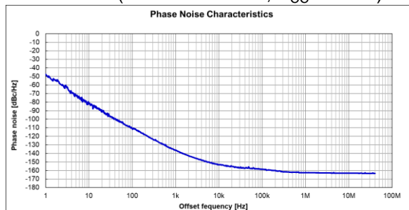
Phase Noise ( f_0 = 156.25 MHz, V_{CC} = 3.3 V)
