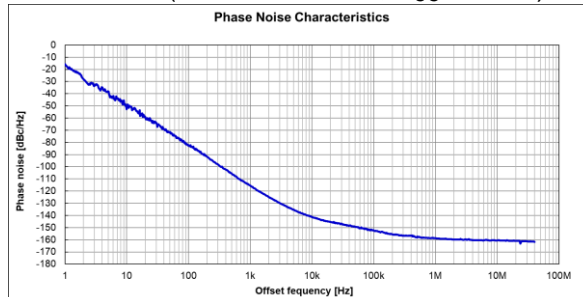
Phase Noise ( f_0 = 491.52 \text{ MHz} , V_{CC} = 3.3 \text{ V} )
