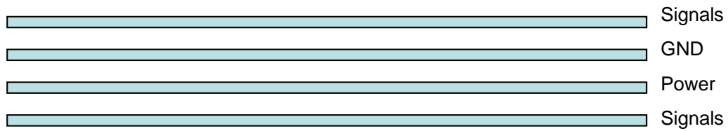
Figure 18: Typical 4-layer PCB construction
