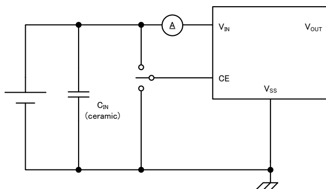
● Circuit ②
