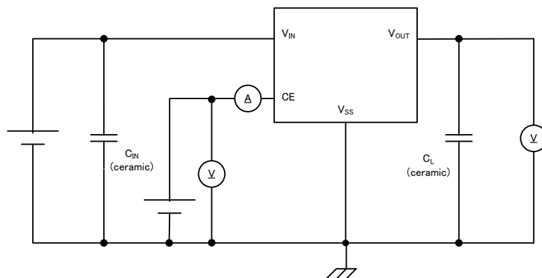
● Circuit ④
