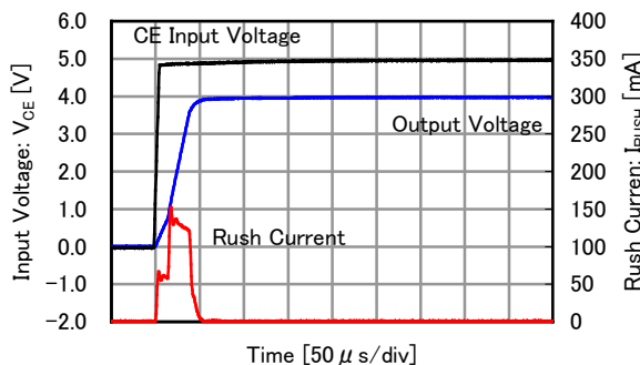
XC6229x401
