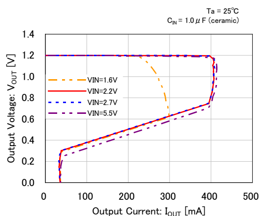
XC6229x121
