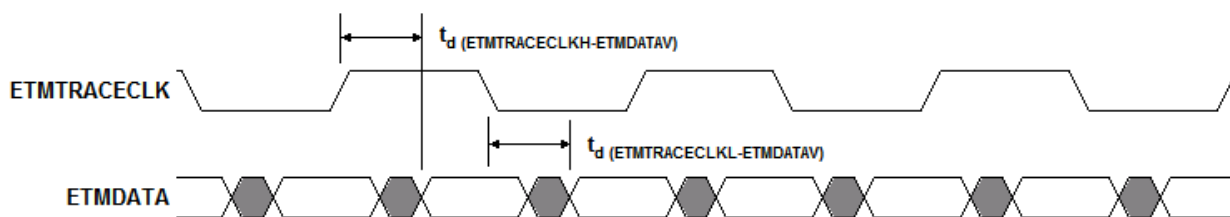
Figure 7-21. ETMDATA Timing
