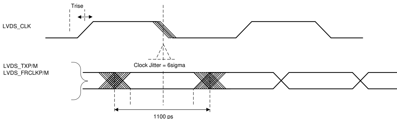
Figure 7-16. Timing Parameters
