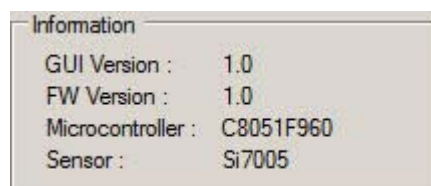
Figure 16. Information Box
