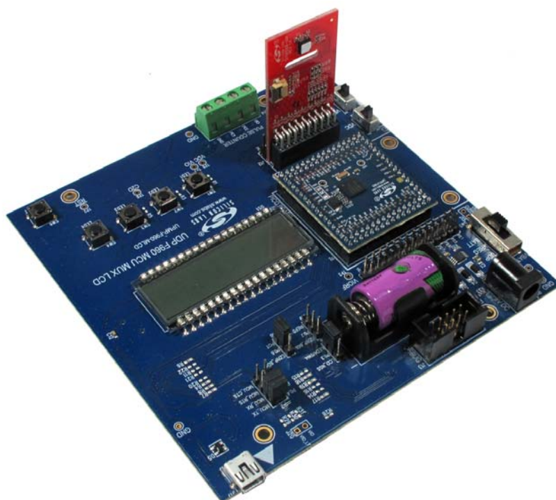
Figure 2. Si7005EB-UDP Port Header Card Plugged into a UDP C8051F960/Si1020 MCU Card with Multiplexed LCD
