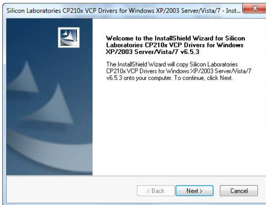
Figure 5. InstallShield Wizard
