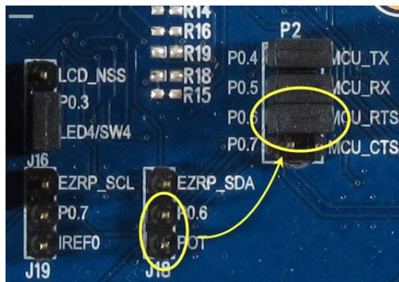
Figure 9. Configuring the MCU Card
