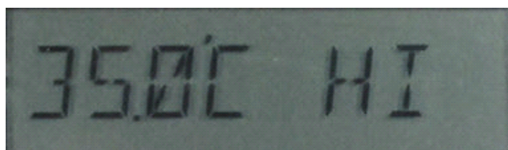
Figure 26. Alarm Display
