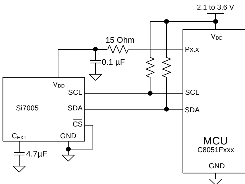
Figure 4. Recommended Connection Diagram for Low-Power Battery Operation
