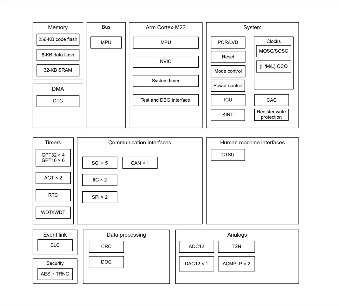
Figure 1.1 Block diagram
