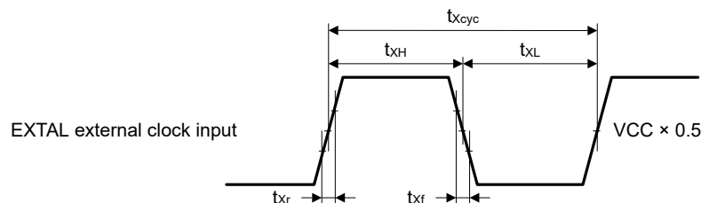
Figure 2.3 EXTERNAL external clock input timing
