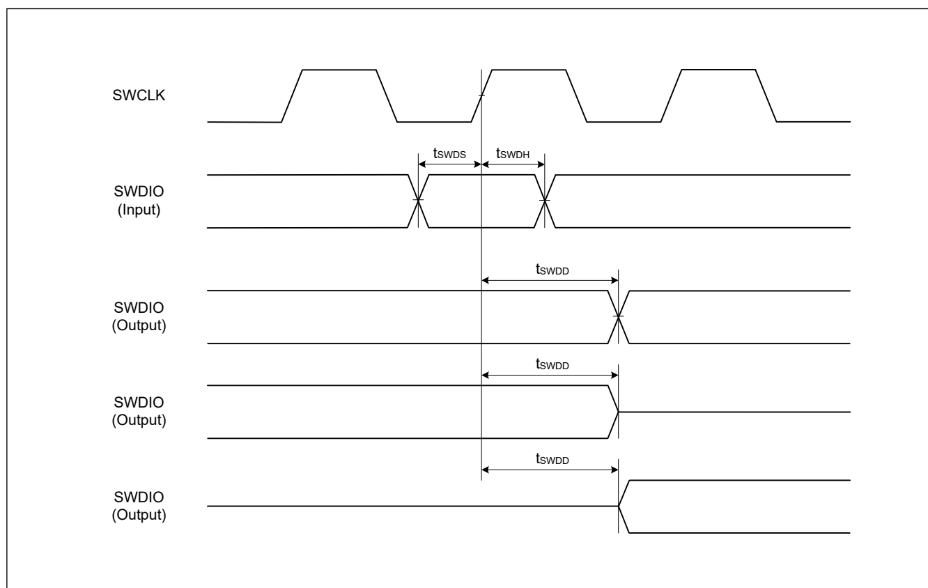
Figure 2.50 SWD input/output timing
