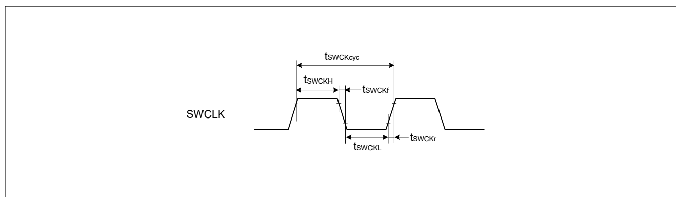
Figure 2.49 SWD SWCLK timing
