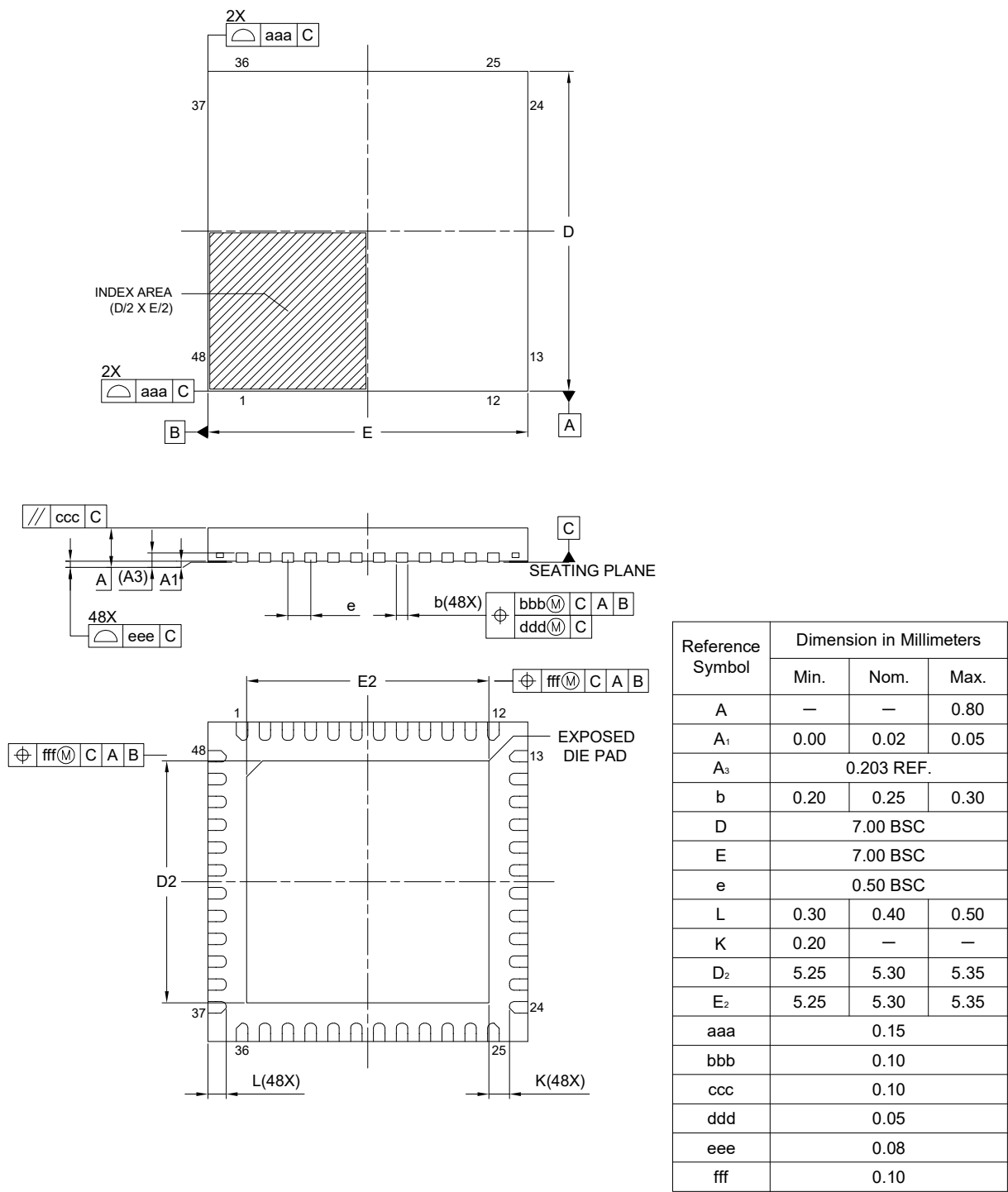
Figure A2.7 HWQFN 48-pin
