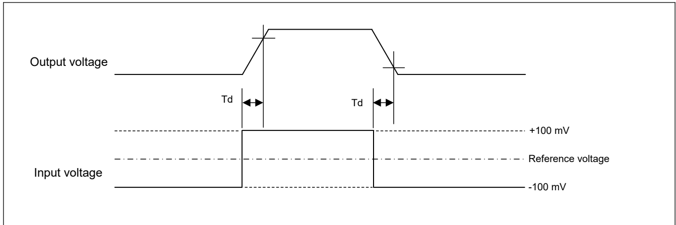
Figure 2.48 Output delay time
