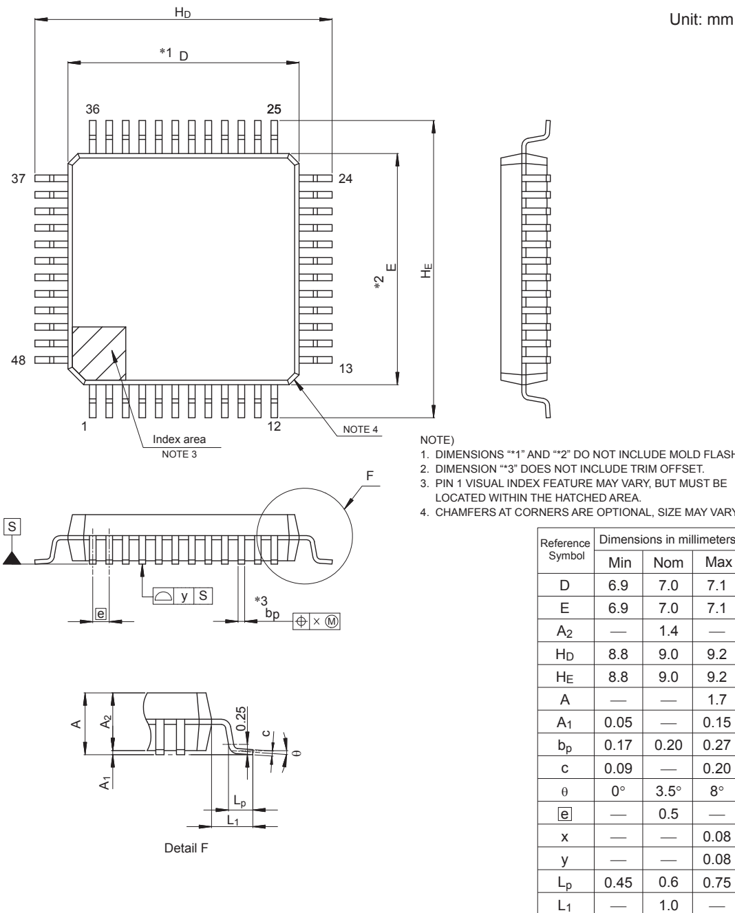
Figure A2.5 LQFP 48-pin (1)
