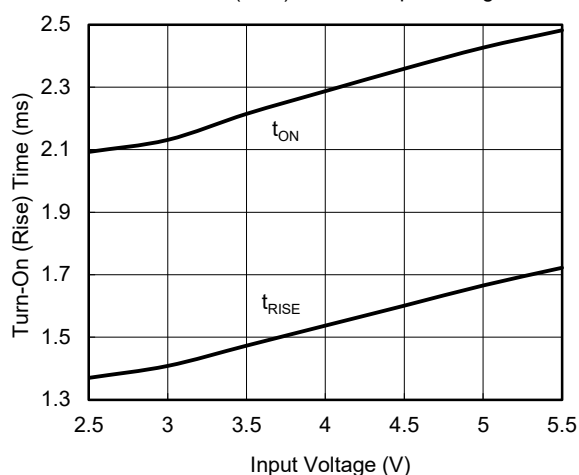
Turn-On (Rise) Time vs. Input Voltage
