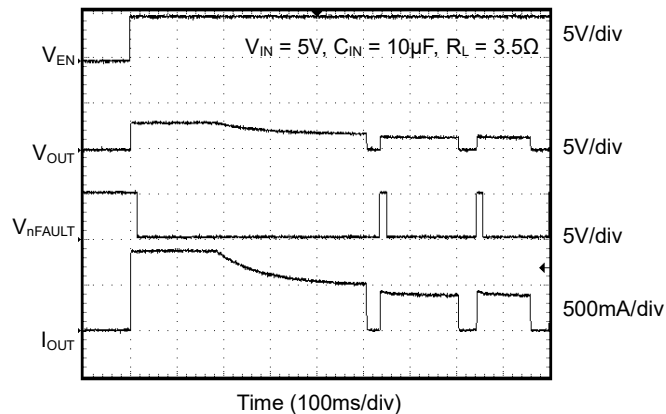
Thermal Shutdown Response (SGM2581A/G)
