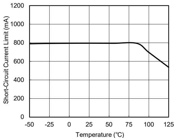
Short-Circuit Current Limit vs. Temperature (SGM2581A/B/G)
