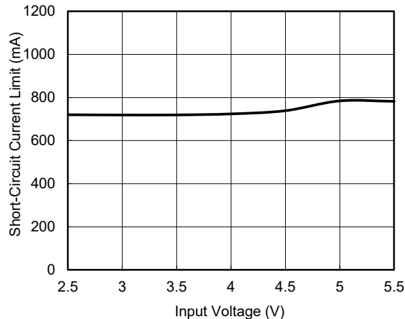
Short-Circuit Current Limit vs. Input Voltage (SGM2581A/B/G)
