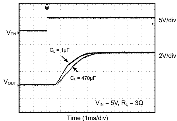
Inrush Current Response (SGM2581C/I)
