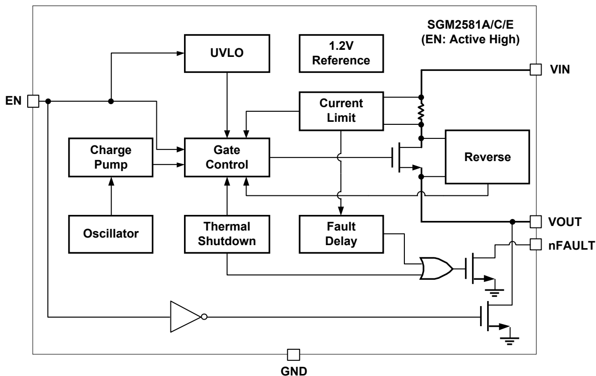
Figure 1. SGM2581A/C/E Block Diagram
