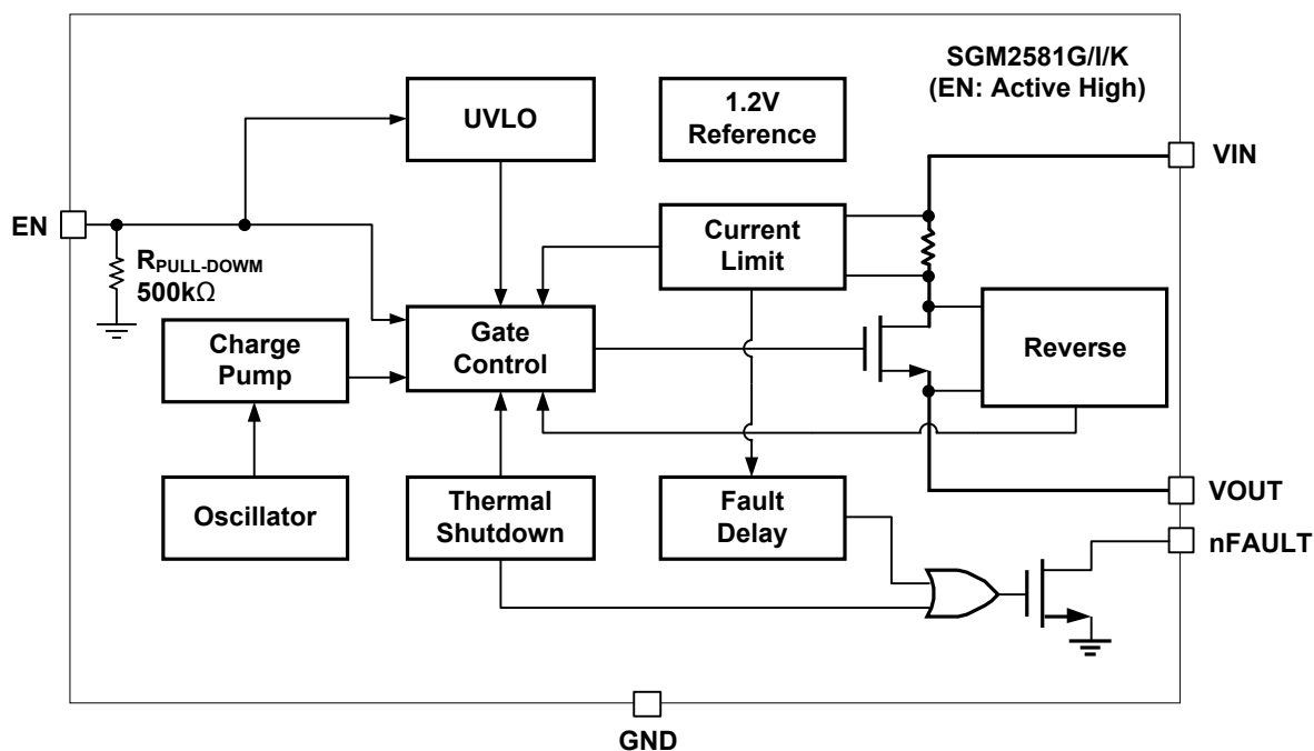
Figure 2. SGM2581G/I/K Block Diagram
