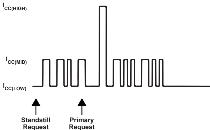
Figure 15: I_{CC(HIGH)} Pulse-Truncating Standstill Pulse Example
