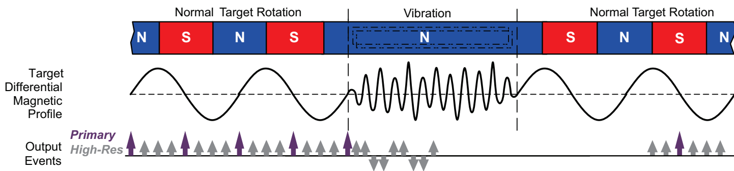
Figure 19: Vibration Behavior
