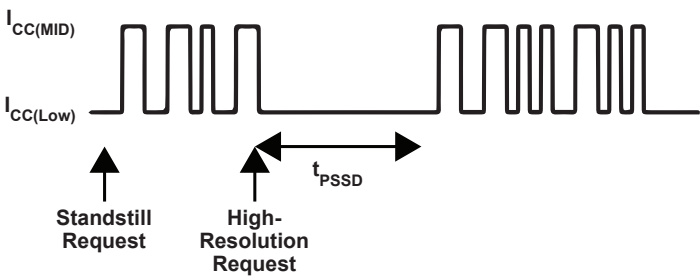
Figure 14: I_{CC(MID)} Pulse-Truncating Standstill Pulse Example, -xAx8 Variant
