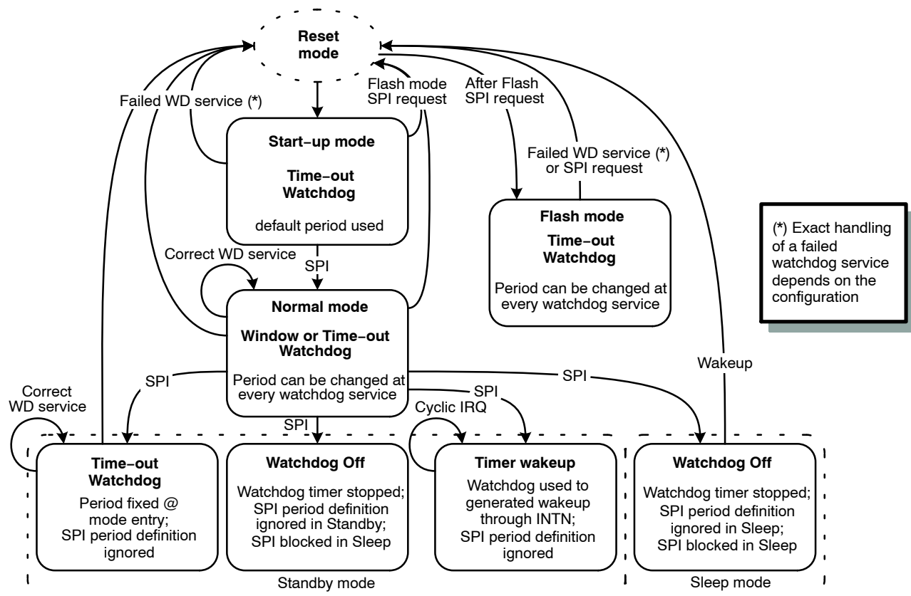
Figure 14. Watchdog Modes
