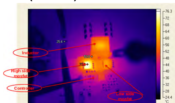
Figure 26. Thermal plot (forced air) Vin=36V Vo=30V, Io=6A fsw=1MHz, TA=25°C
