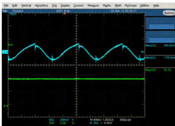
Figure 33. Ripple at 1MHz Vin=48V, Vo=30V, Io=10A Lo=1μH, Co=12μF ceramic
