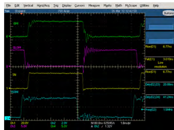
Figure 14. Gate drive and switching node fsw=1.5MHz, Io=7A
