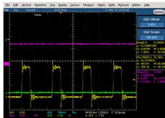
Figure 41. Steady state operation Vin=12, Vo=3.3V 5MHz No load Ch1 (yellow): Switching node, Ch3 (purple): Vout, CH4 (green): Io
