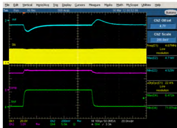
Figure 39. Transient step response Vin=24V, Vo=5V 5MHz 1-7A, Fc=140kHz Ch1 (yellow): Switching node, Ch2 (blue): Vo, Ch3 (purple): COMP, CH4 (green): Io
