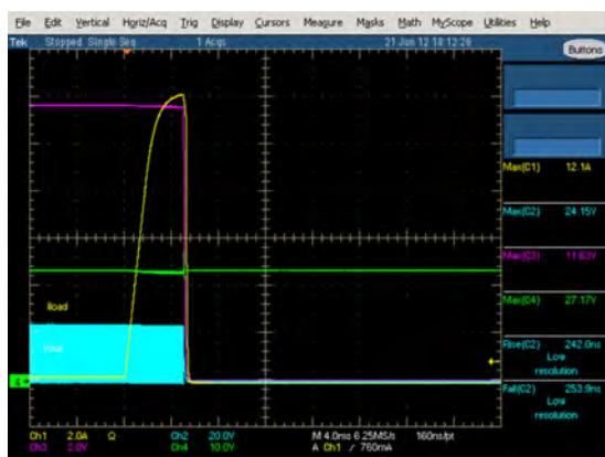
Figure 17. Current limit operation R_{ds\_on} = 13m\Omega , R_{lim} = 128k\Omega Ch1 (yellow): output current, Ch2 (blue): switching node Ch3 (purple): output voltage, Ch4 (green): input voltage
