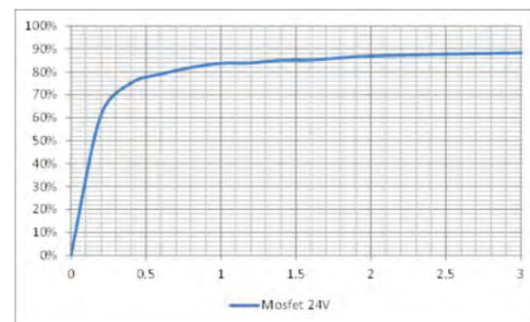
Figure 28. 2.5MHz Vo=12V efficiency with MOSFET BSC123N08NS3G
