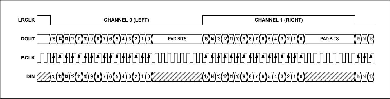
Figure 2. Left-Justified Mode
