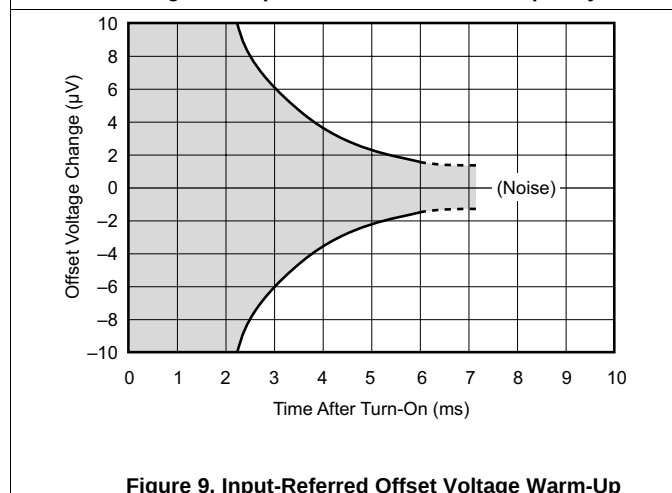
Figure 9. Input-Referred Offset Voltage Warm-Up
