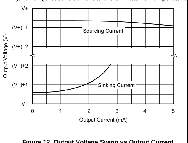
Figure 12. Output Voltage Swing vs Output Current
