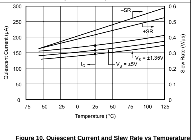
Figure 10. Quiescent Current and Slew Rate vs Temperature
