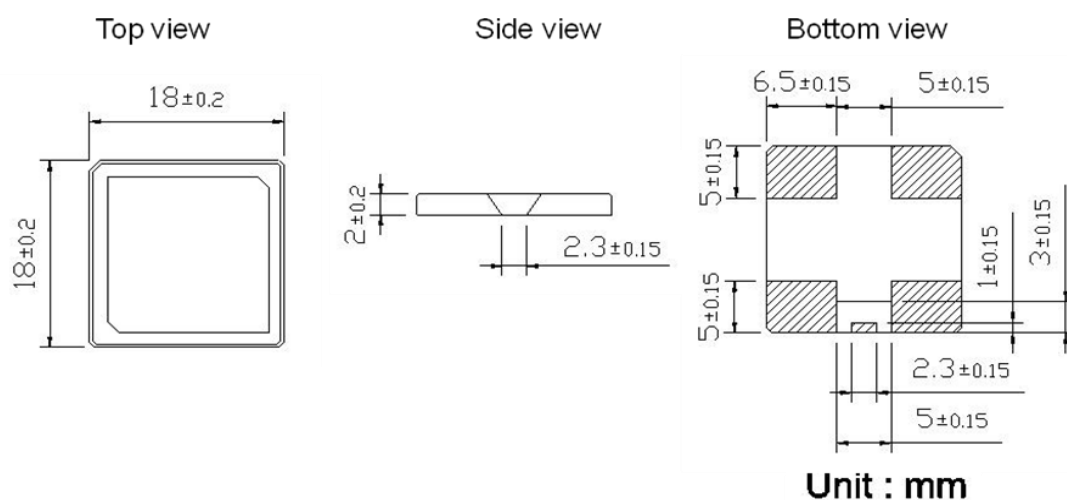
Fig. 1 Mechanical data
