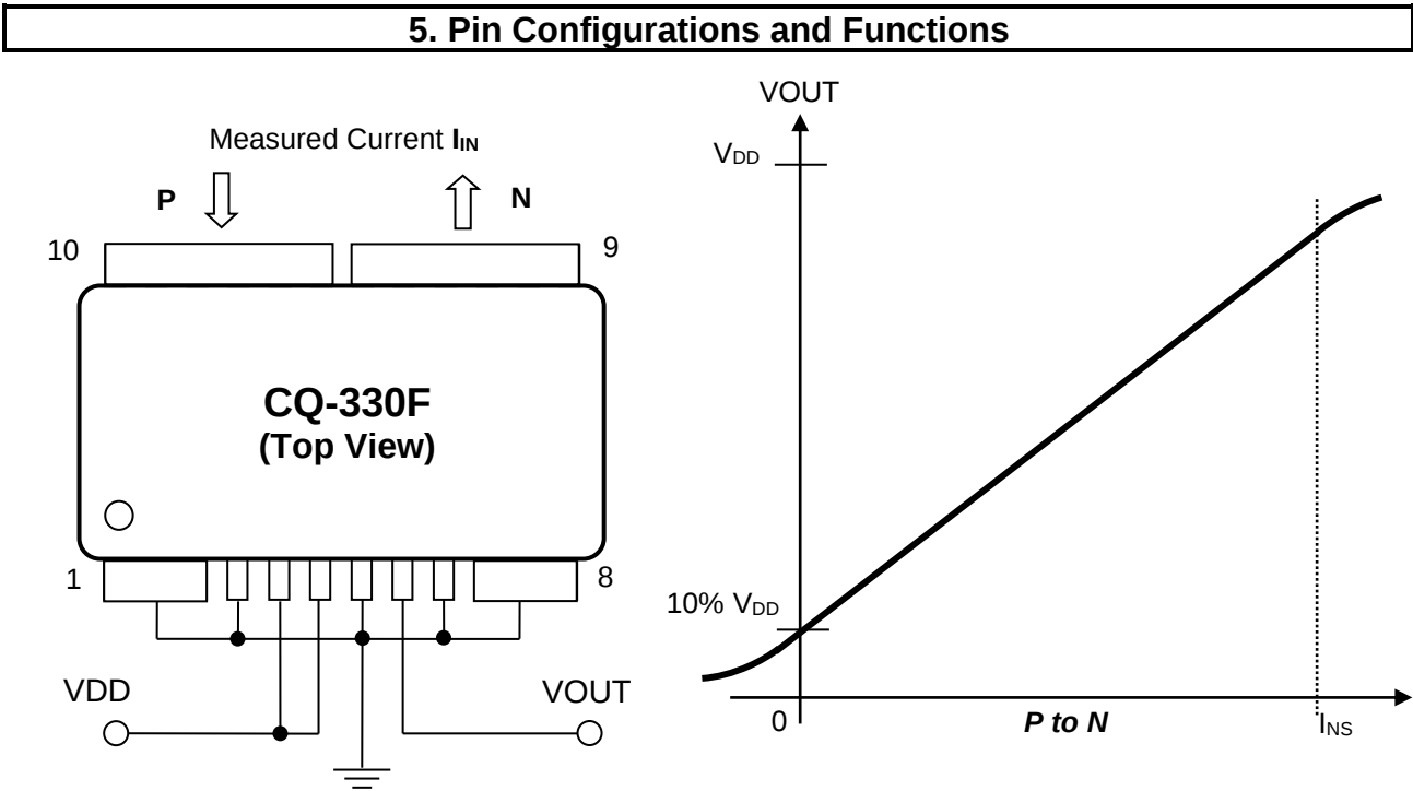
Figure 2. Pin assignment and typical output characteristics of CQ-330F
