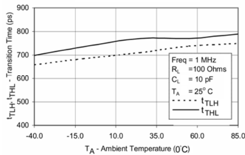
Figure 20. Transition Time vs. Ambient Temperature
