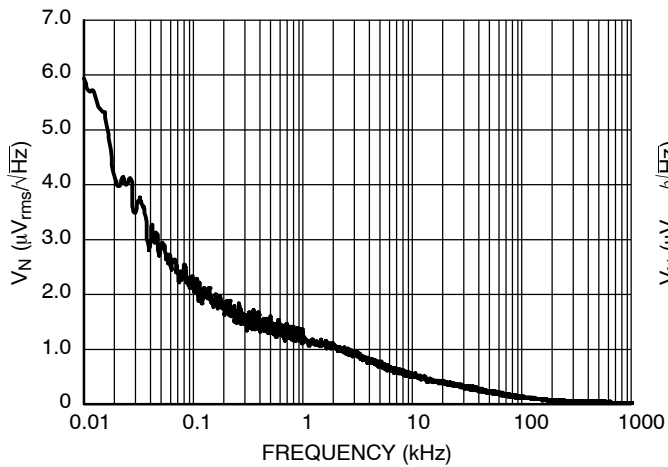
Figure 33. Output Voltage Noise, 2.8 V Version, V_{IN} = 3.8 V , I_{OUT} = 30 mA
