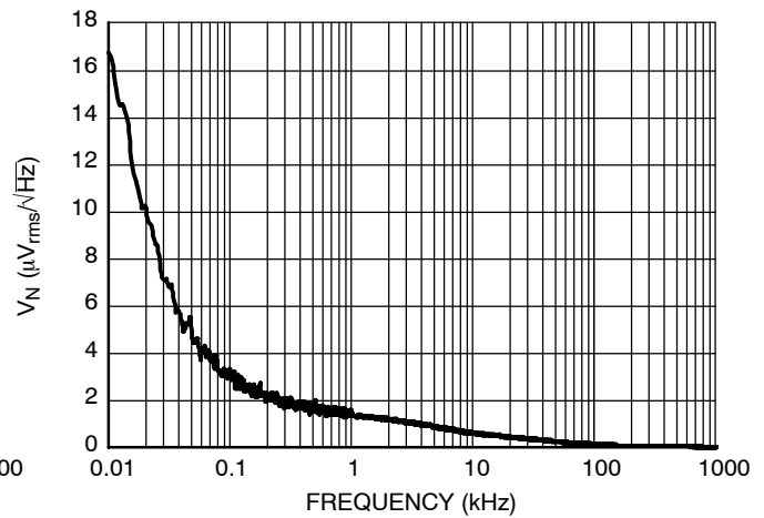
Figure 34. Output Voltage Noise, 3.3 V Version, V_{IN} = 4.3 V , I_{OUT} = 30 mA
