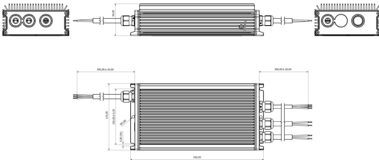
Figure 3. Mechanical drawing
