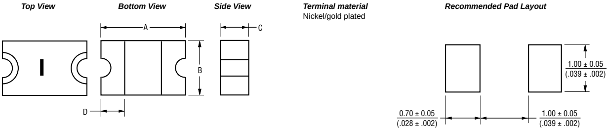
Product Dimensions
