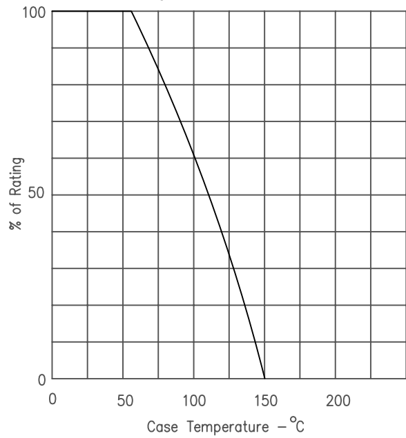
Figure 3 Current Derating
