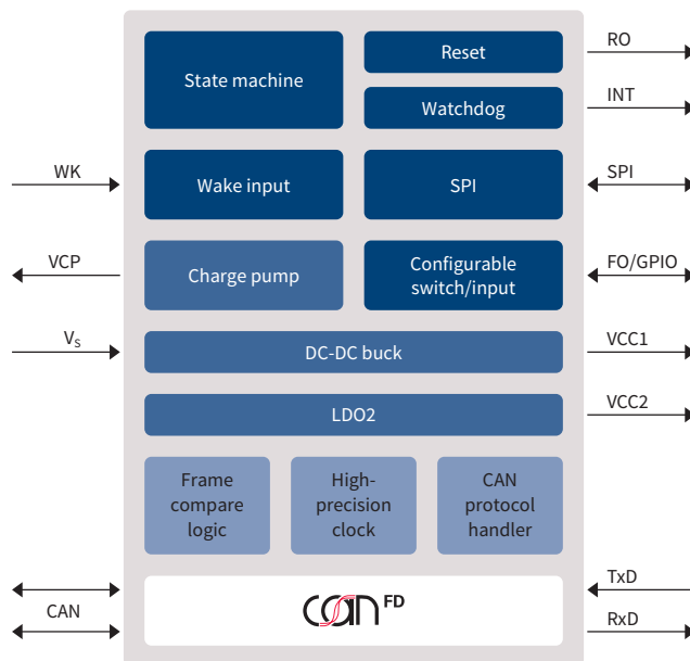
Block diagram TLE9471
