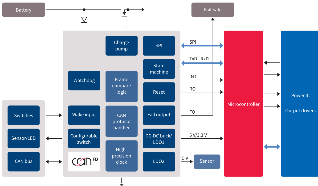
Application diagram TLE9461/71
