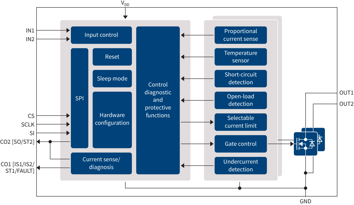
Block diagram TLE8102SG
