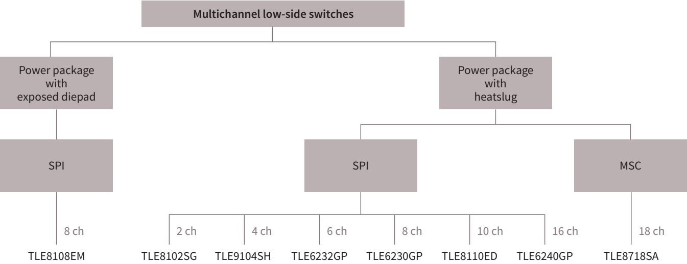
Selection tree – multichannel low-side switches
