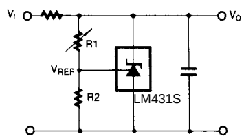
Figure 13. Shunt Regulator
