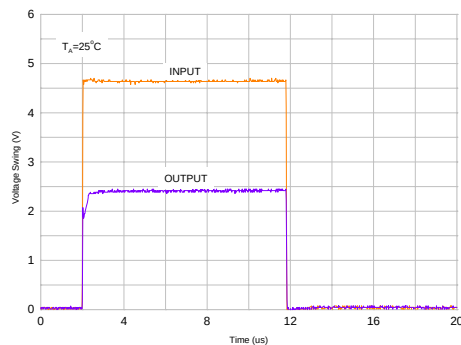
Figure 9. Pulse Response
