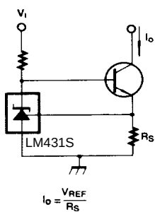
Figure 17. Constant-Current Sink
