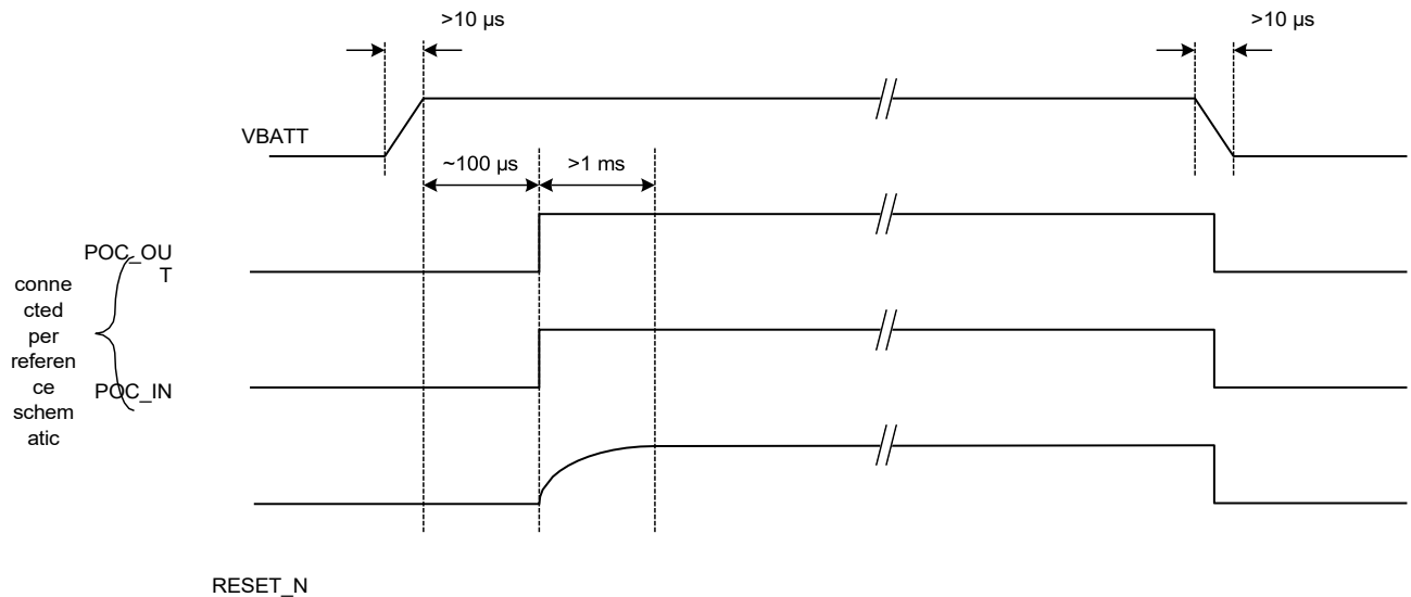
Figure 7.1. Power Up Sequence
