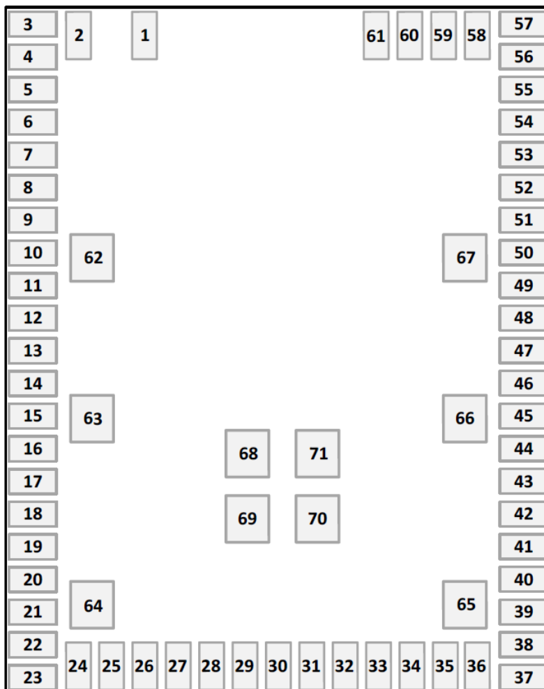
Figure 9.2. Pin Numbering
