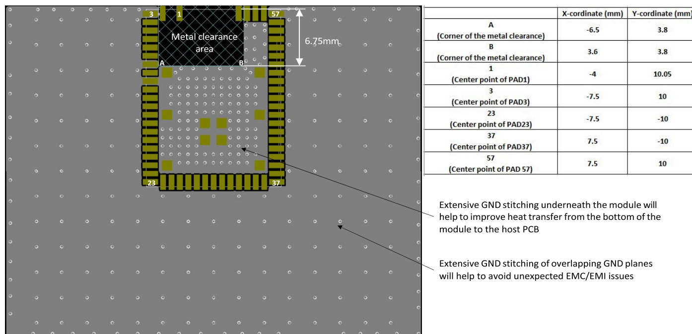
Figure 8.34. Application Layout of 453-00222
