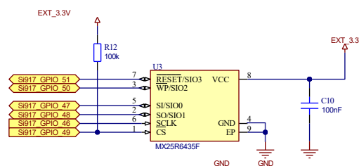
Figure 8.9. Option 4: External 3.3 V Common Flash (NWP + MCU) Powered From External 3.3 V Supply
