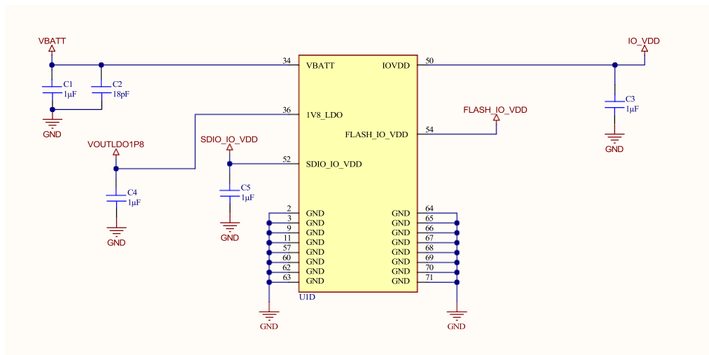
Figure 8.16. System Power Supplies
