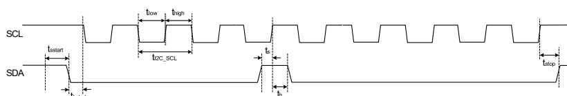
Figure 7.14. Interface Timing Diagram for I2C High Speed Mode
