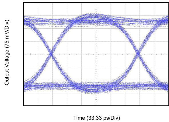
Figure 6-10. USB 3.1 Gen1 Eye-Pattern Performance with 12-inch Input PCB Trace at 5 Gbps
