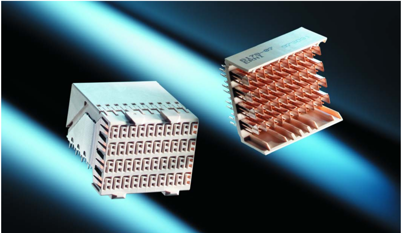
ERmet ZD Male and Female Module with Pressfit Termination
