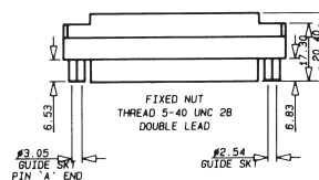
SOCKET – FIXED NUT
