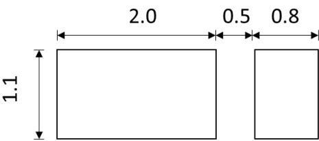
Fig. 9.1 Land Pattern Dimensions (for reference only) (Unit: mm)
