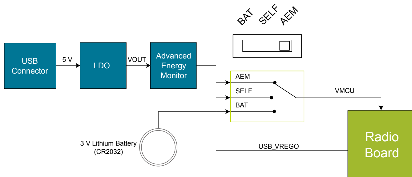
Figure 4.1. Power Switch
