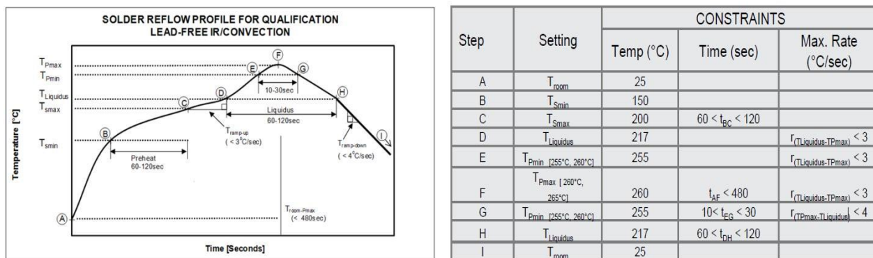
Figure 10-1 Solder Reflow Profile
