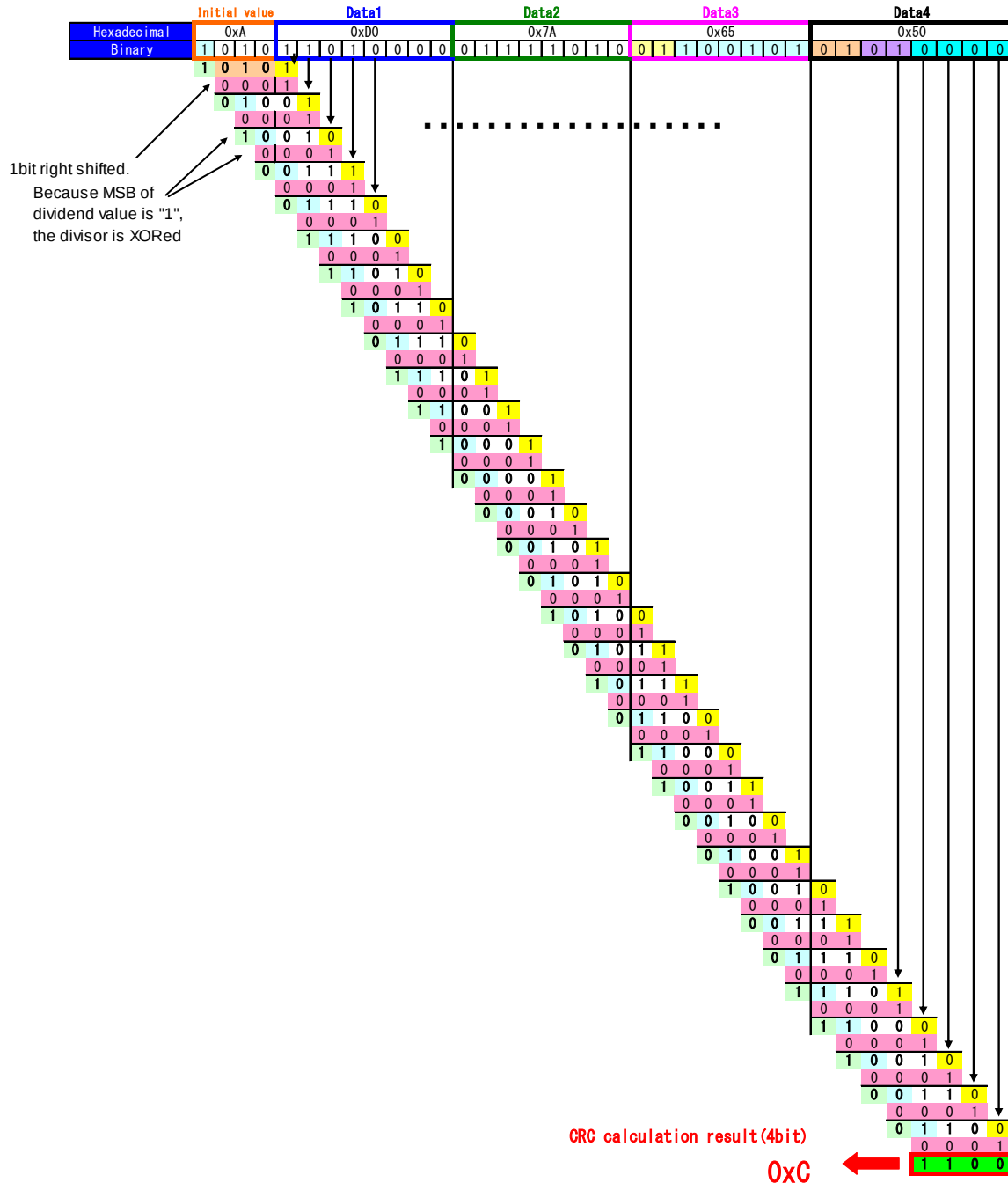
Figure 5-6 CRC Calculation
