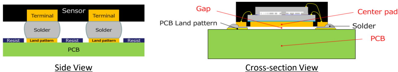
Figure 10-2 Solder Joint
