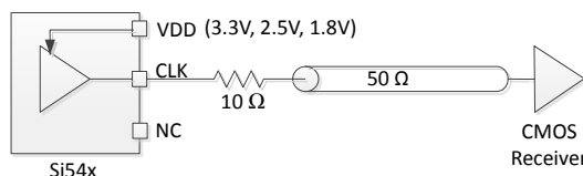
Single CMOS Termination
