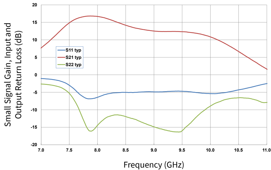
Figure 1. Small Signal Gain and Return Loss vs Frequency of CGHV96050F1 measured in CGHV96050F1-AMP
