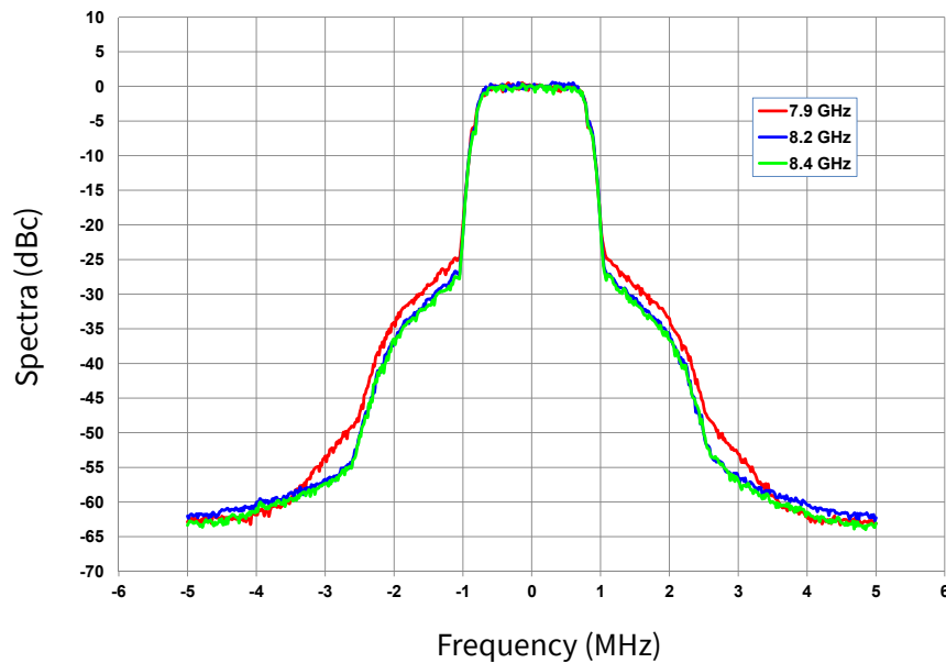
Figure 7. Spectral Mask under QPSK Modulation, 1.6 Msps V_{DD} = 40\text{ V} , Output Power = 44 dBm / 25 W
