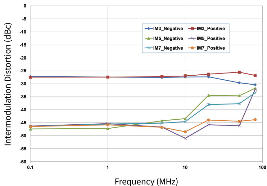
Figure 2. Intermodulation Distortion Performance vs. Tone Spacing
