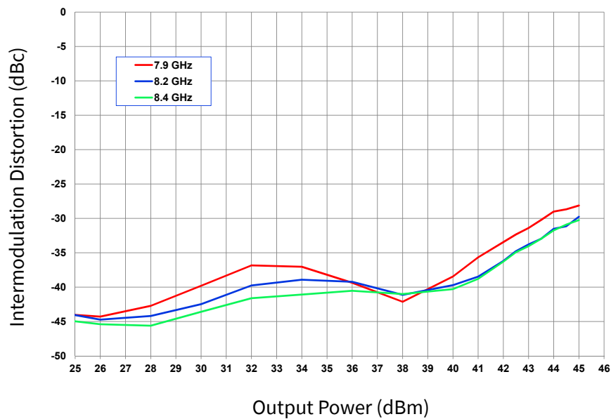
Figure 9. OQPSK Linearity vs Output Power
