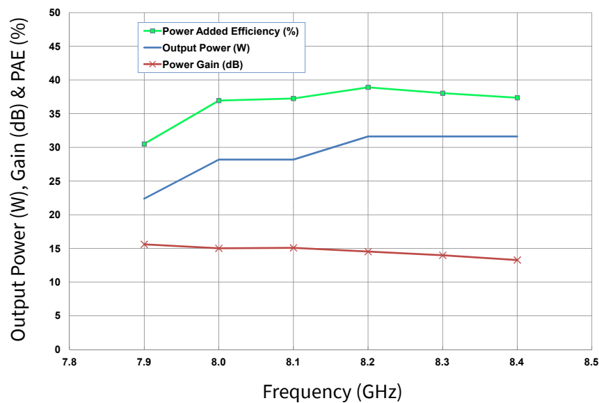
Figure 8. Linear Output Power, Gain, and Power Added Efficiency vs Frequency V_{DD} = 40\text{ V} , I_{DQ} = 500\text{ mA} , 1.6 Msps, QPSK Modulation at -30 dBc
