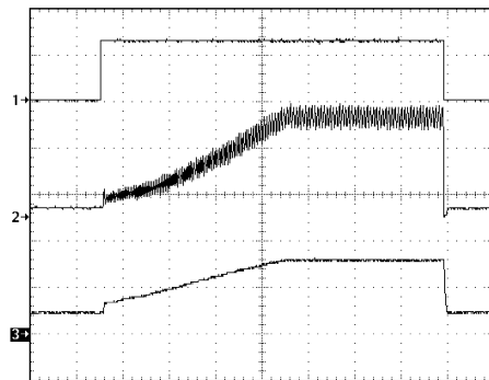
Figure 38. T_A = 85^\circ\text{C}
