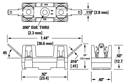
Q.C. Terminals Type: 05200003Z
