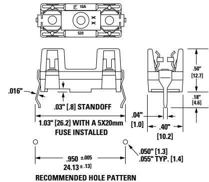
PC Board Mount Type: 05200006ZXGR
