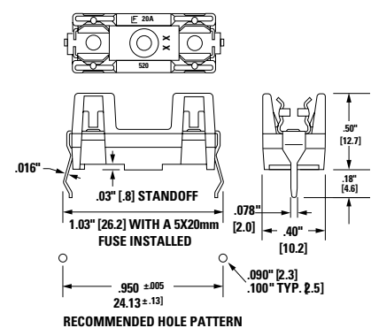
PC Board Mount Type: 05200006ZXGR
