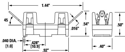
Solder Terminals Type: 05200010ZXBLU
