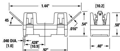
Q.C. Terminals Type: 05200005ZXGY
