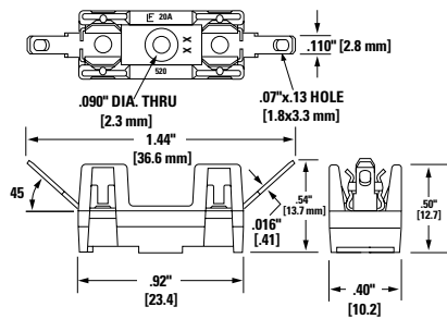
Solder Terminals Type: 05200004Z 05200008ZXGR
