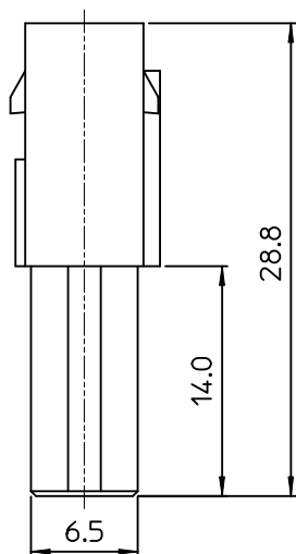
VIEW A
