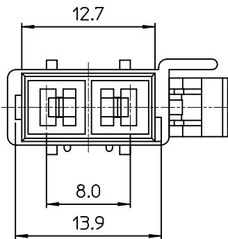
VIEW A
