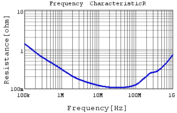
RCER71H103K0K1H03B R DCOV, 25degC
