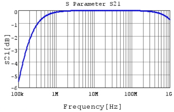
RCER71H103K0K1H03B S21 DC0V, 25degC
