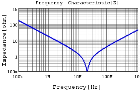
RCER71H103K0K1H03B |Z| DCOV, 25degC
