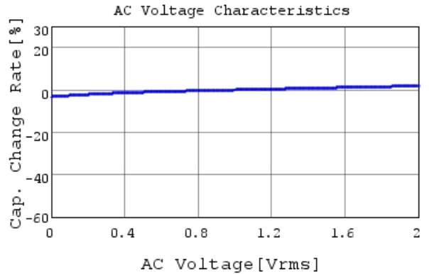
RCER71H103K0K1H03B C-AC Voltage capchange, I
