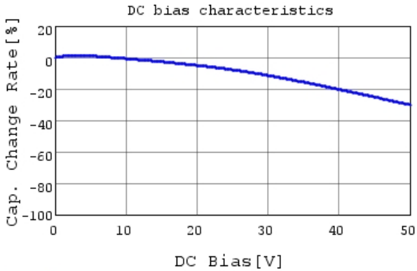
RCER71H103K0K1H03B C-DC bias capchange, 25.0
