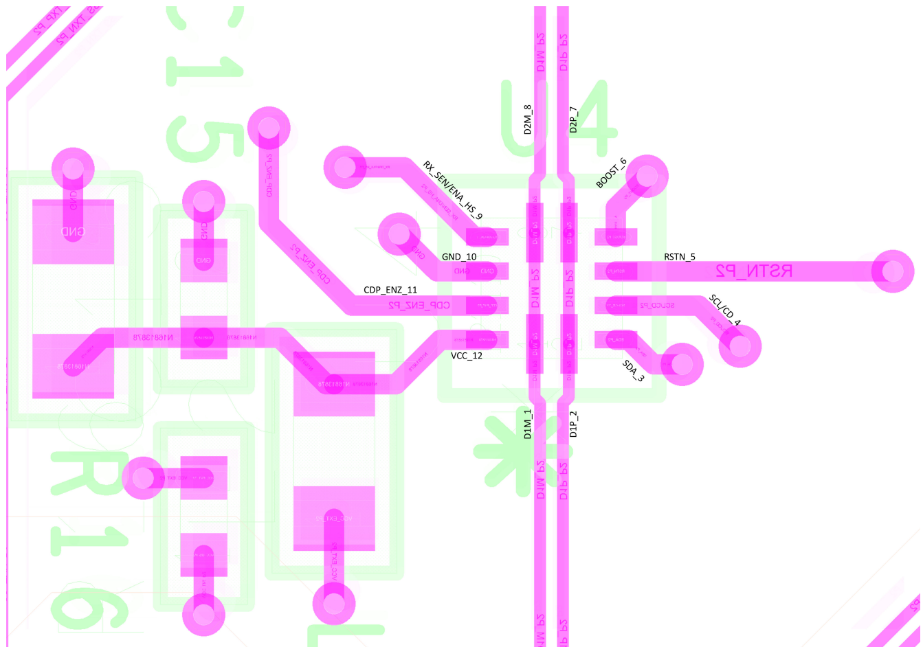
Figure 8-22. Layout Example
