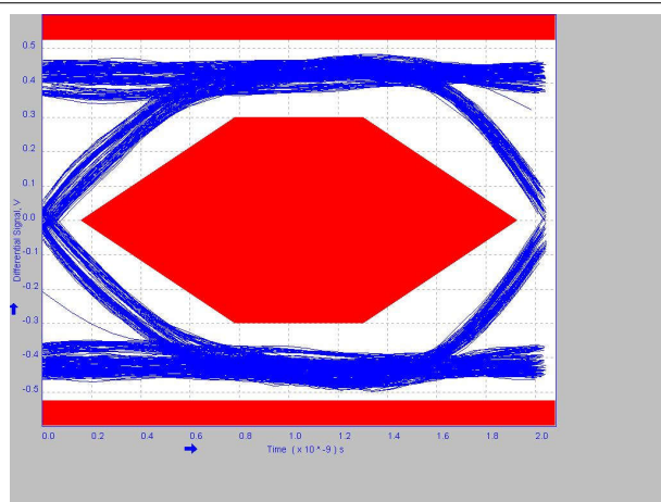
Figure 8-5. 2 Meter Pre-Channel With TUSB216 BOOST=0 RX_SEN=HIGH
