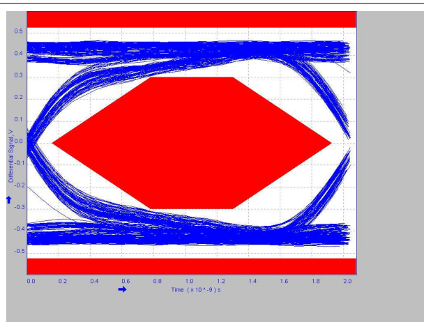
Figure 8-3. 2 Meter Pre-Channel Without TUSB216
