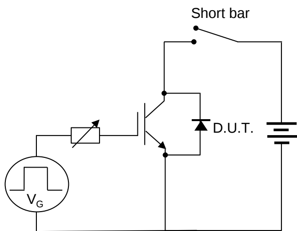
Fig.30 Short Circuit
